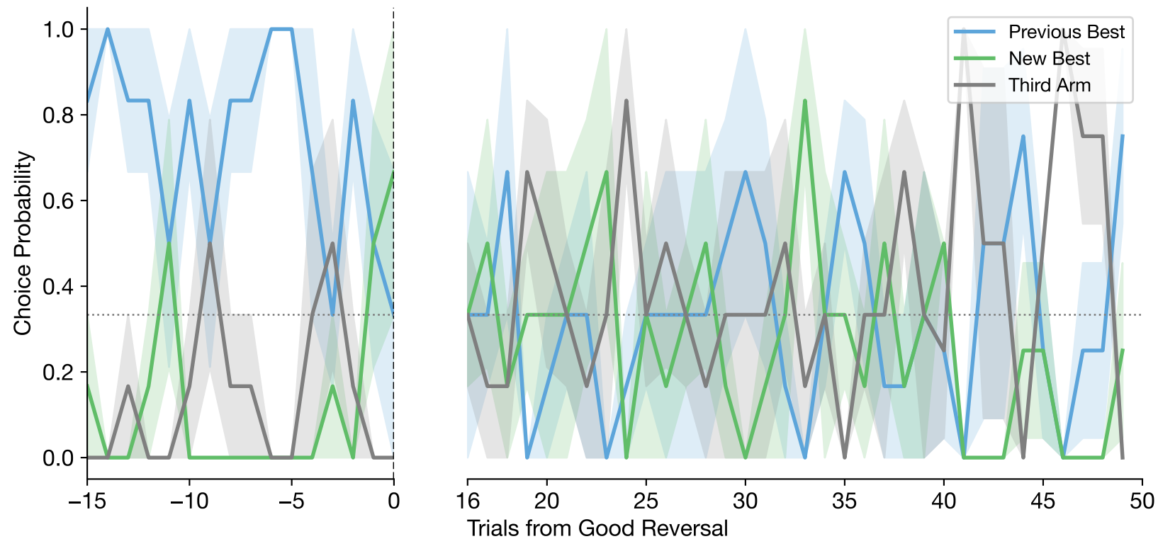
Good Reversal-Aligned Choices (mean \pm se across subjects | n=3 subjects, n=5 reversals) (Skipping first 15 trials post-reversal)
